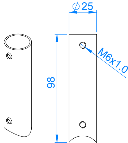
2PCS. Ø25 X 98 MM S.STEEL DOUBLE GRUB SCREW MOUNTING LEG
