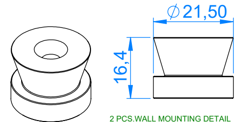
2 PCS.WALL MOUNTING DETAIL MATERIAL ALUMINIUM 6063 T5
