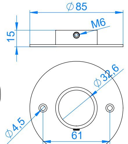
1 PCS. Ø85 X 15 mm S.STEEL MOUNTING FLANGE
